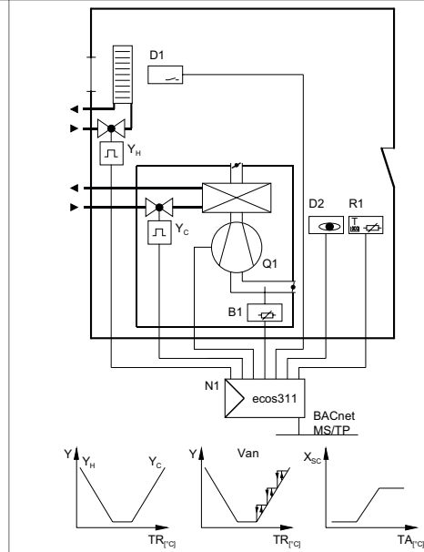
Fan coil temperature controller with 4-pipe system Heating with radiator
